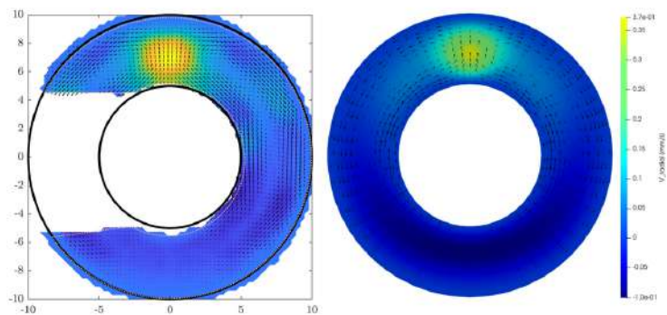
Figure 1: Experimentally measured radial velocity (left), steady finite element solution (right) for \Delta T = 2 K and V_{peak} = 8 kV.
