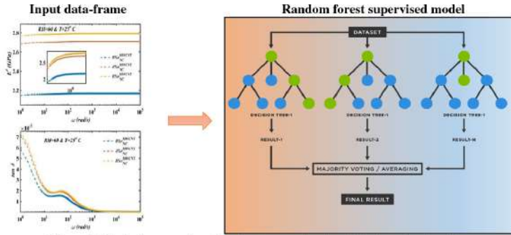
Figure 1 Block diagram of random forest supervised machine learning algorithm
